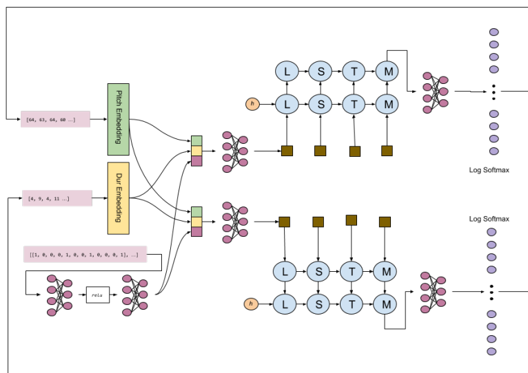
Fig. 3: This figure displays a diagram of the full system described above, showing two mirrored, interdependent LSTM networks, each concatenating the other's output to its own input along with the current chord to condition their generations. The concatenation of pitch, duration and chord sequences is encoded by each network before being fed to their respective LSTM layers.
